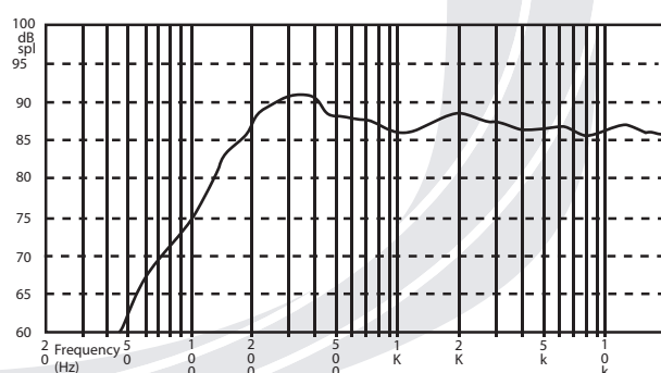
Frequency Response between 150 Hz and 20 KHz
