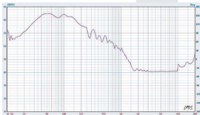
Frequency Response between 30 Hz and 180 KHz
